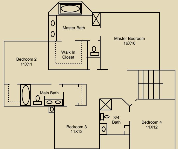
Upper Level
