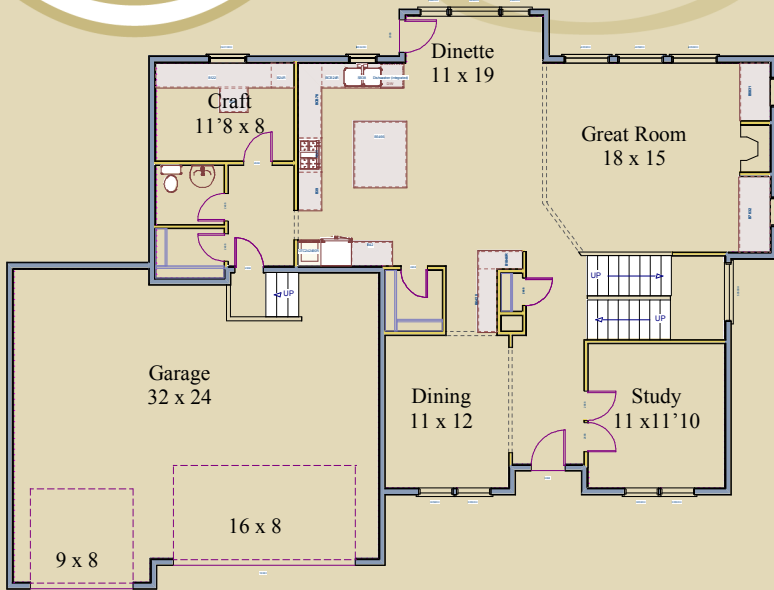
Main Level
