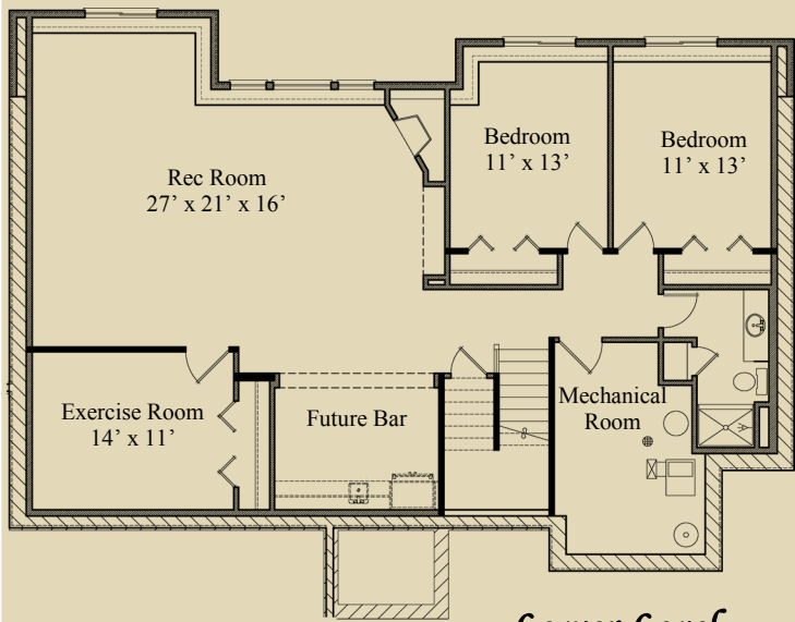
Lower Level
